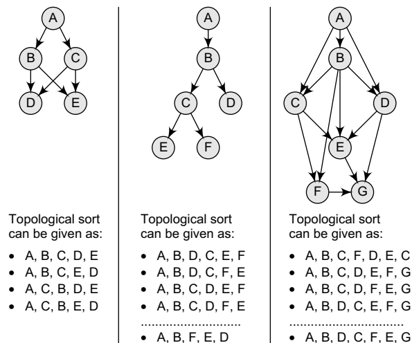
Figure 13.24 Topological sort
